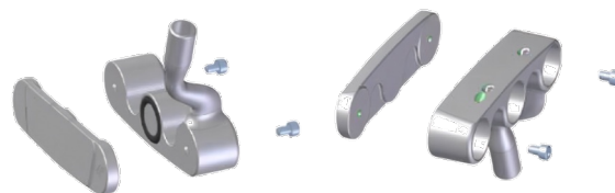
Interchangeable loft angle face plates.
